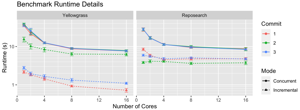
Fig. 31. Absolute runtimes of WebDSL benchmarks
