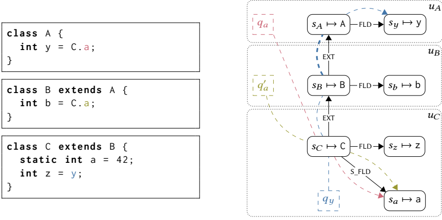
Fig. 15. Example demonstrating unsound confirmation. References are colored similar to the queries they correspond to. The resolution step with thick dashes between s_B and s_A indicates a transitive dependency.
