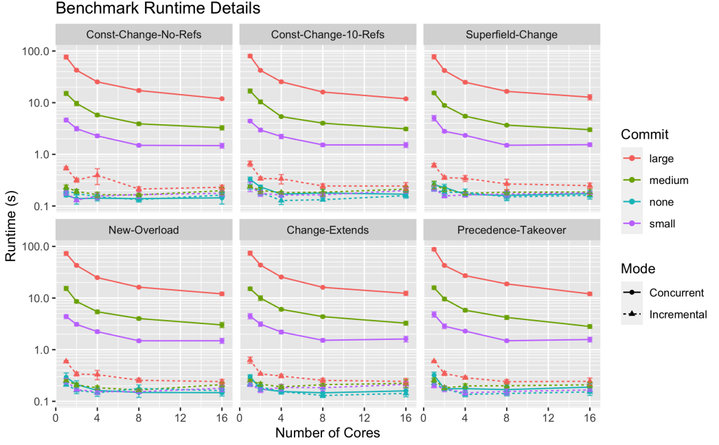
Fig. 32. Absolute runtimes of synthetic benchmarks
